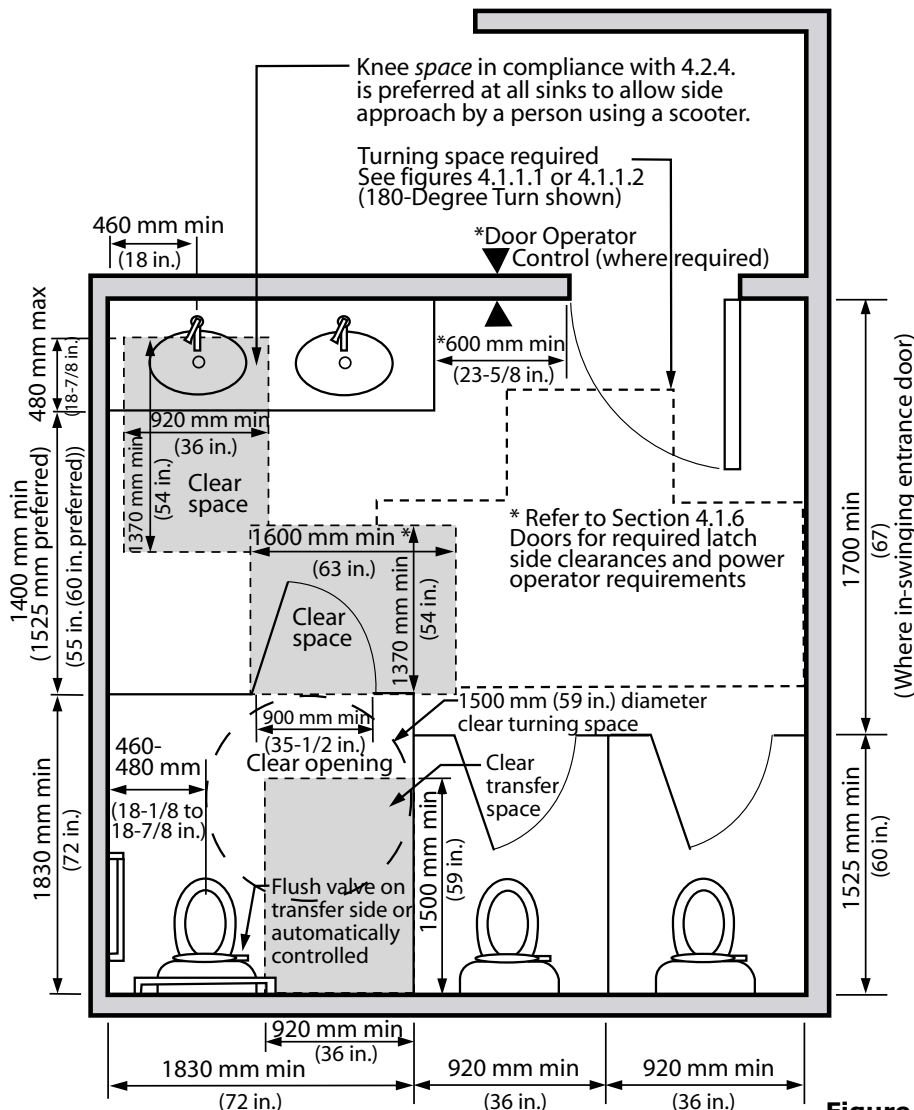
Figure 4.2.1.1 Washroom Dimensions
