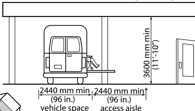
Figure 4.3.13.1 Clearances at Passenger Loading Zone
