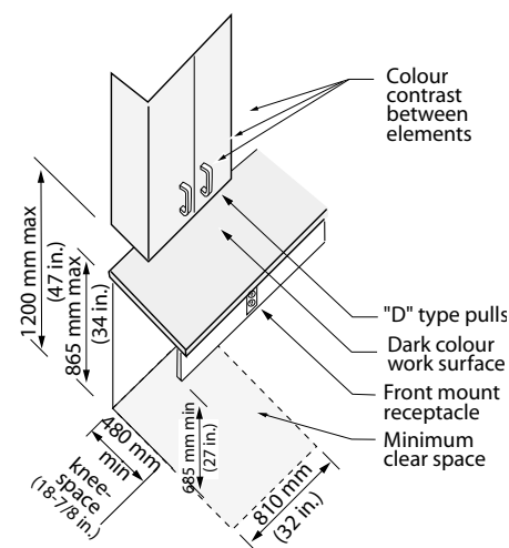
Figure 4.3.18.4 Storage Elements
