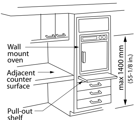
Figure 4.3.18.8 Wall-Mounted Oven
