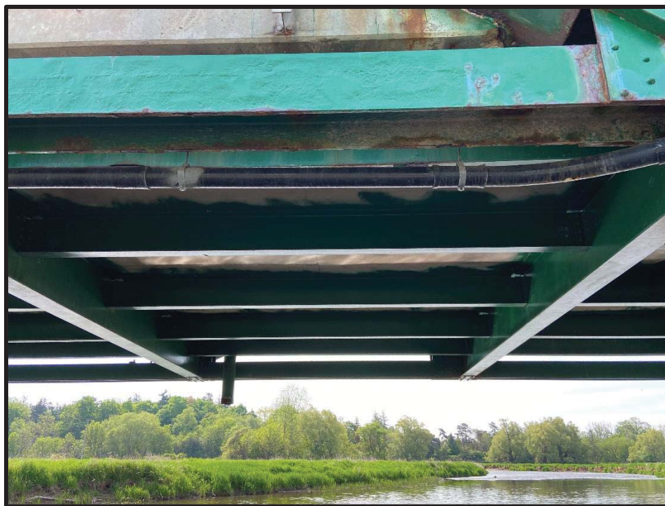
Image 29: Underside Detail of Stringers, Old Derry Road Bridge (May 27, 2020; View looking Southeast)
