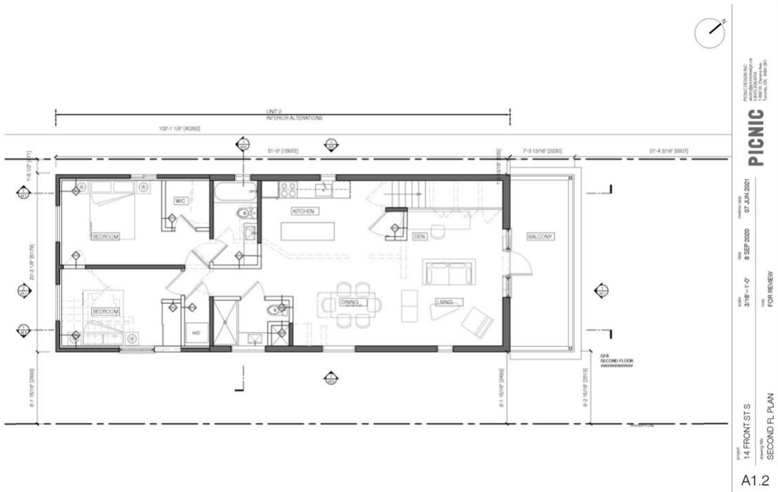
Second Floor Plan n.t.s.
