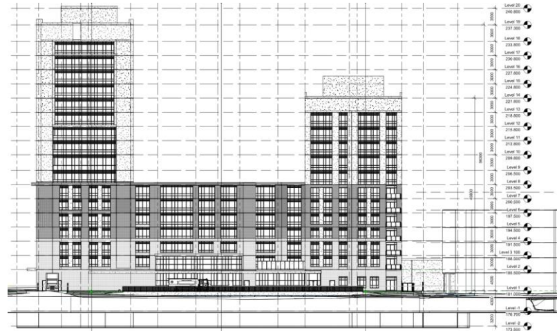
West Elevation
