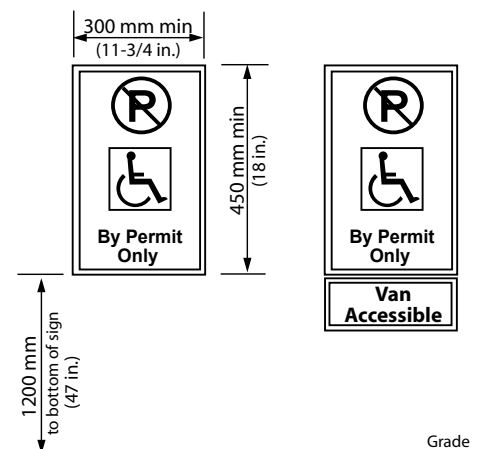
Figure 4.3.12.3 Regulatory Parking Signage
