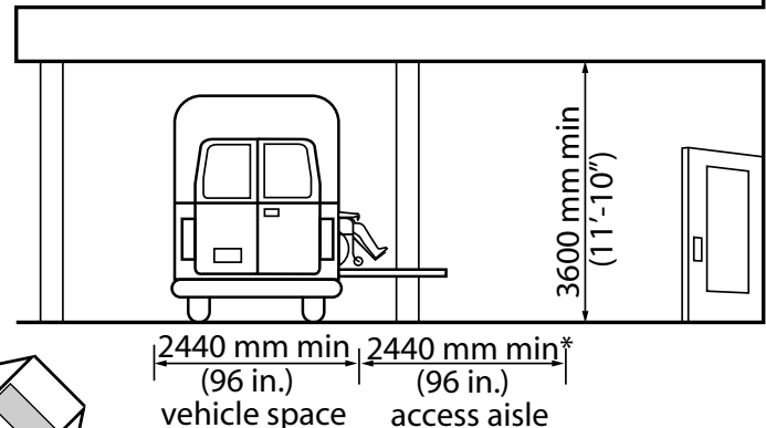
Figure 4.3.13.1 Clearances at Passenger Loading Zone
