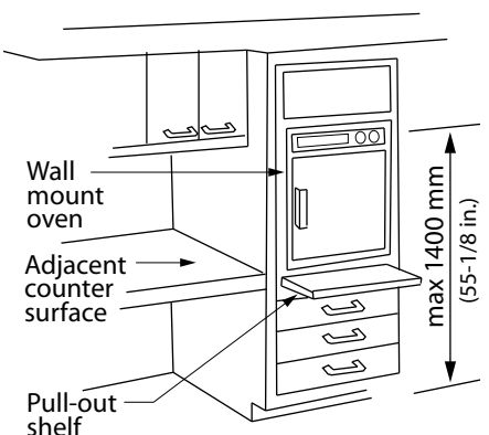
Figure 4.3.18.8 Wall-Mounted Oven
