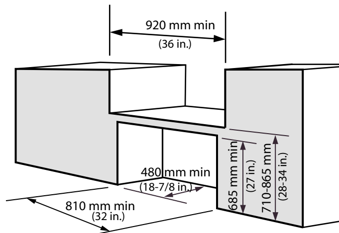
Figure 4.3.8.1 Service Counter
