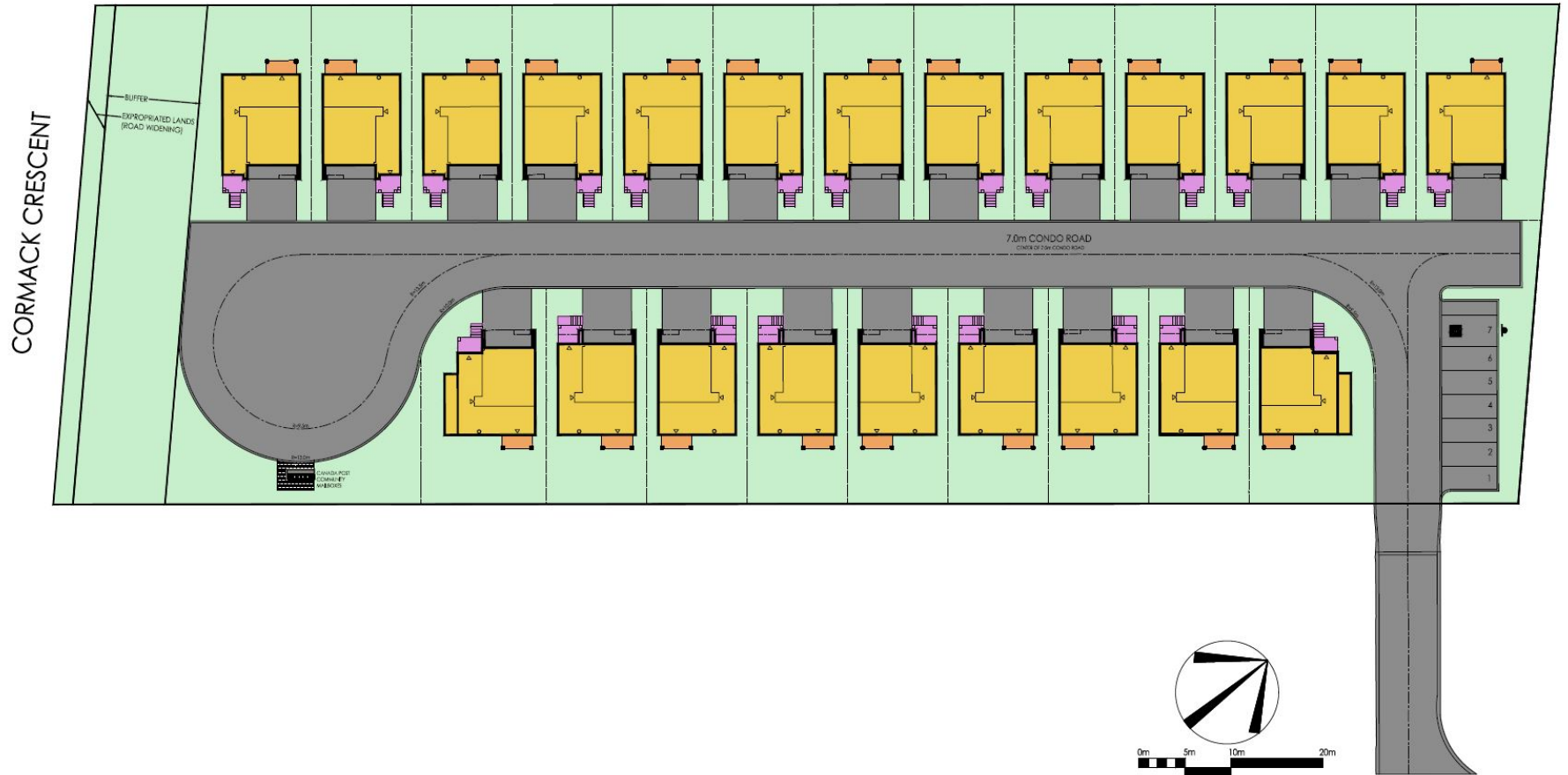
Site Plan
