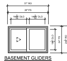
BASEMENT GLIDERS SCALE: 3/4" = 1'-0"
