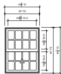
30X40 SINGLE HUNG 2ND FLOOR SCALE: 3/4" = 1'-0"
