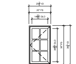
GUEST SUITES 2ND FLOOR REAR SCALE: 3/4" = 1'-0"
