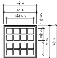
30X30 SINGLE HUNG 2ND FLOOR SCALE: 3/4" = 1'-0"
