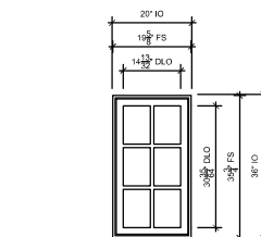
GUEST SUITES 2ND FLOOR REAR SCALE: 3/4" = 1'-0"
