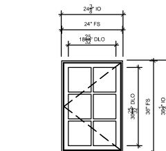
GUEST SUITE 2ND FLOOR REAR SCALE: 3/4" = 1'-0"
