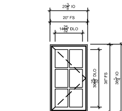
GUEST SUITES 2ND FLOOR REAR SCALE: 3/4" = 1'-0"
