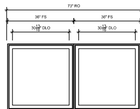
3RD FLOOR TOWER SCALE: 3/4" = 1'-0"
