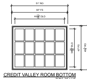
CREDIT VALLEY ROOM BOTTOM SCALE: 3/4" = 1'-0"
