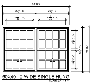
60X40 - 2 WIDE SINGLE HUNG SCALE: 3/4" = 1'-0"
