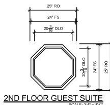
2ND FLOOR GUEST SUITE SCALE: 3/4" = 1'-0"
