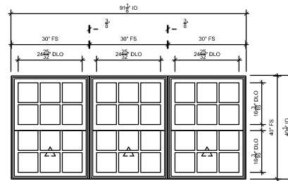
3 WIDE SINGLE HUNG SCALE: 3/4" = 1'-0"
