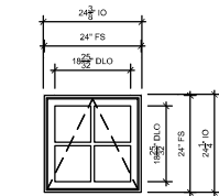
2ND FLOOR AWNING SCALE: 3/4" = 1'-0"
