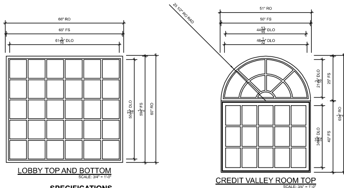
LOBBY TOP AND BOTTOM SCALE: 3/4" = 1'-0"
