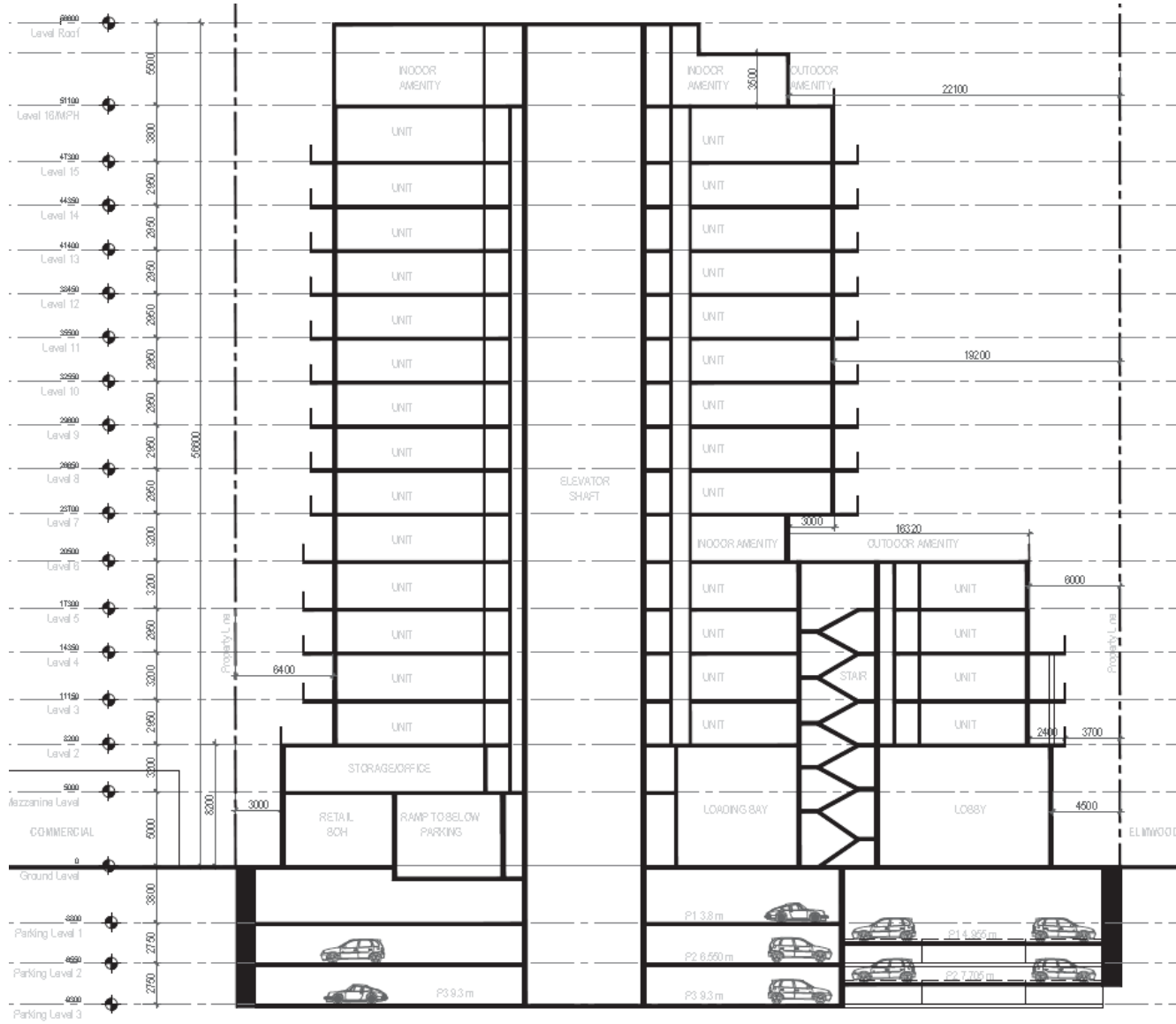
Cross Section of Building
