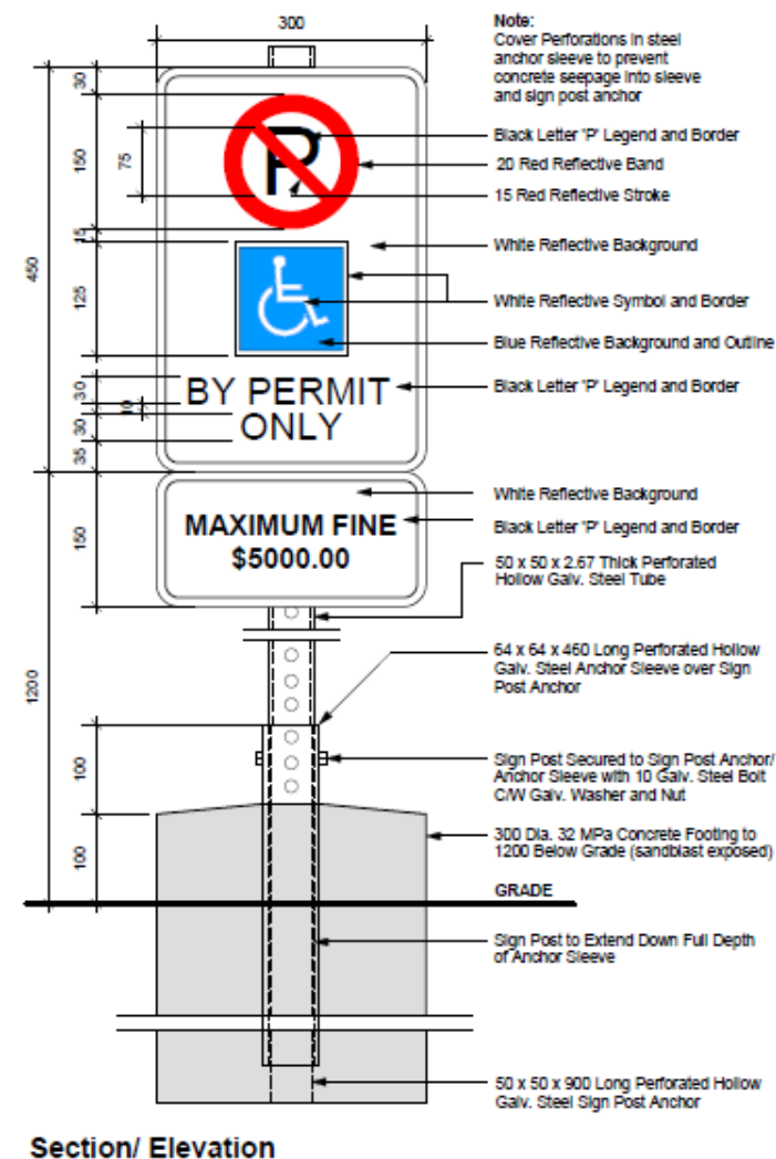
DETAIL 3 - Accessible Sign Scale NTS
