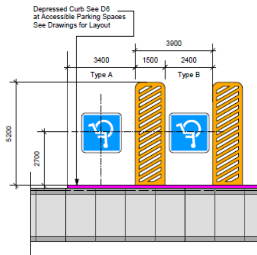
Plan 5.2m Type A and B Parking Stalls
