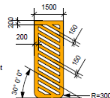
Typical Painting Detail
