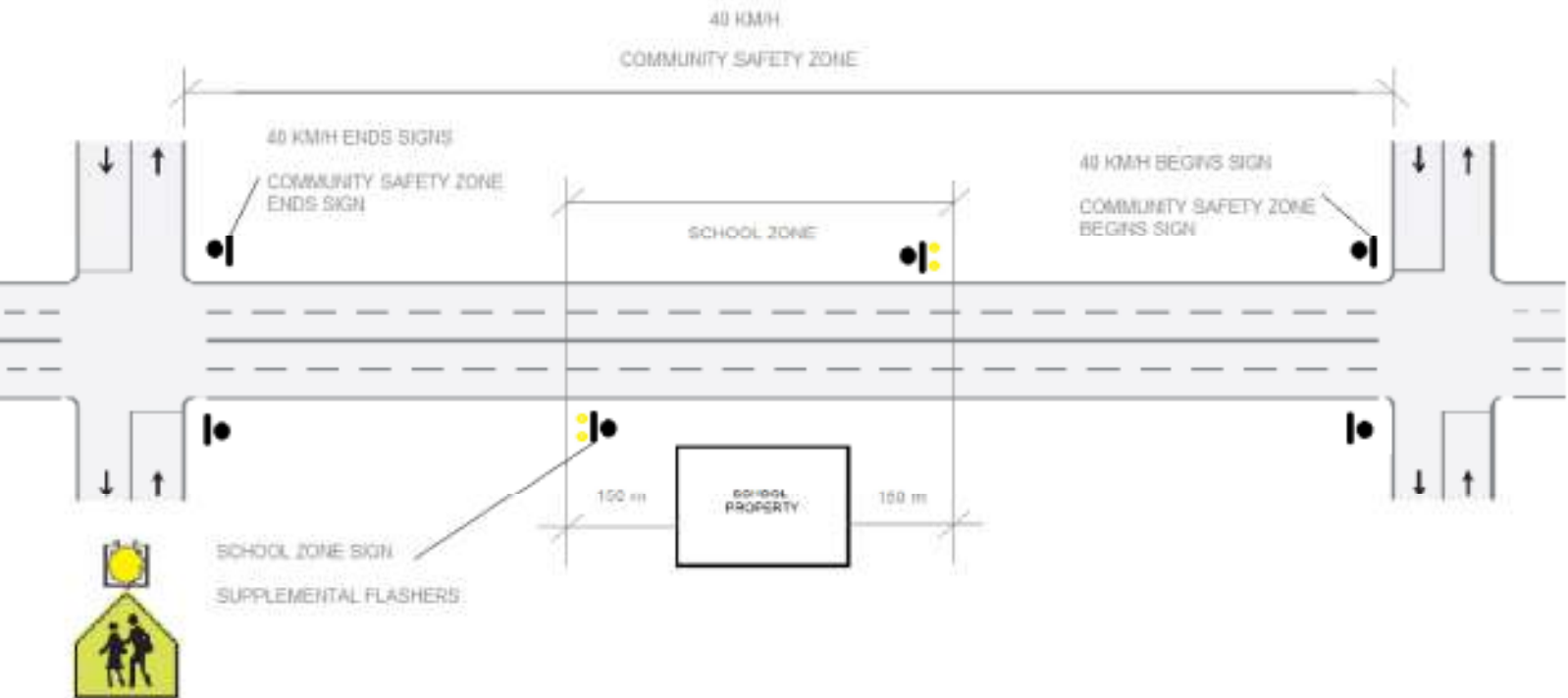
TYPICAL SCHOOL ZONE LAYOUT - PROPOSED
