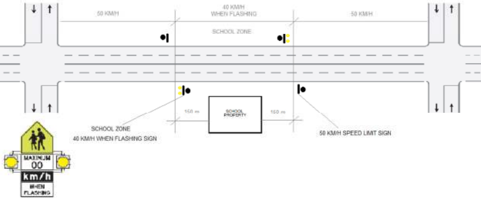
TYPICAL SCHOOL ZONE LAYOUT - EXISTING
